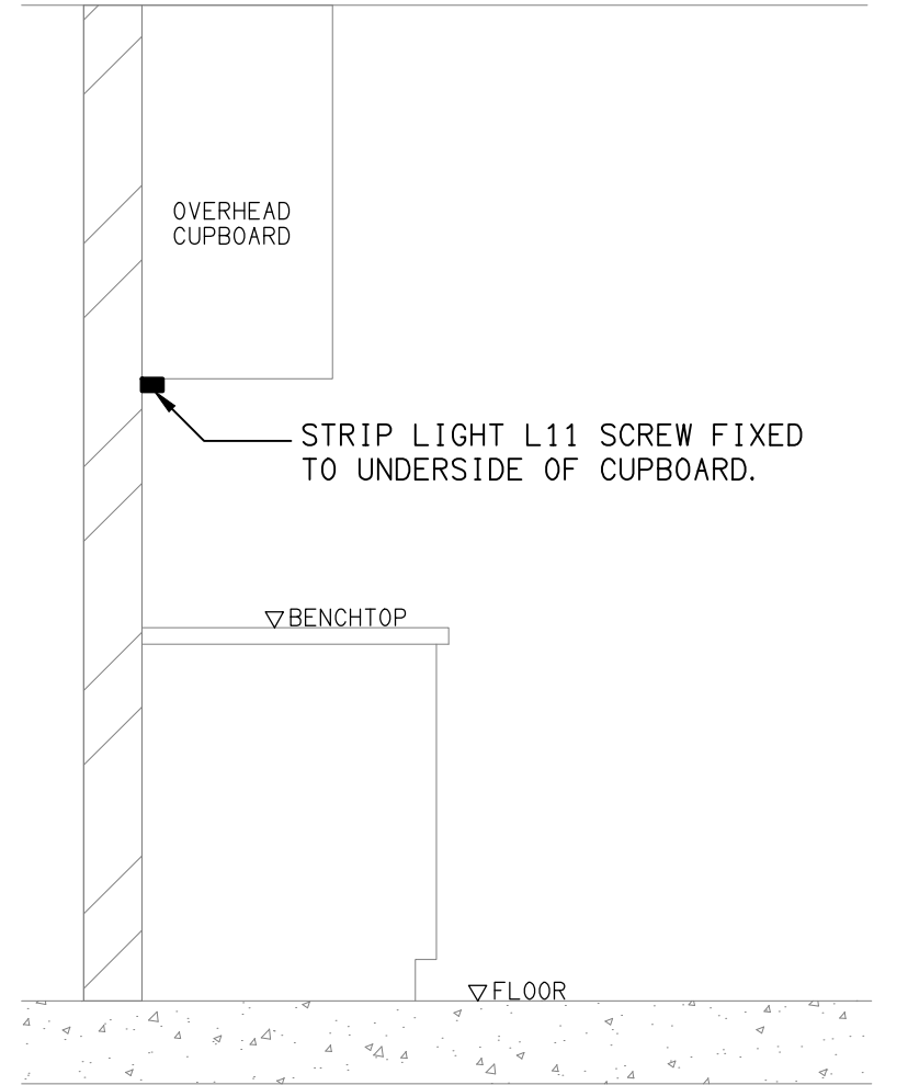
DETAIL "L11" TYPE STRIP LIGHT MOUNTING NOT TO SCALE
